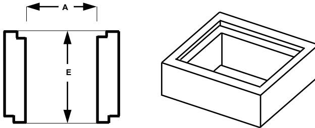
CONCRETE PIT RISERS – TABLE OF DIMENSIONS (mm)
