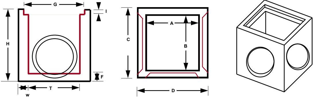
CONCRETE PIT BASES – TABLE OF DIMENSIONS (mm)
